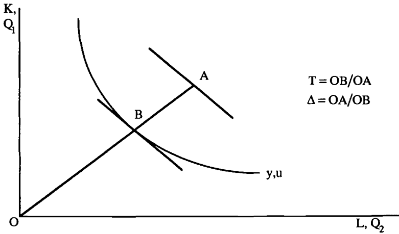
Fig. 8.1 The distance function
