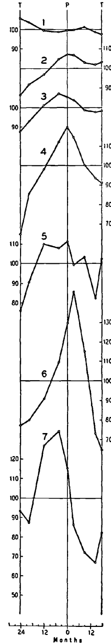
Seven cycles during downswings (1927-33 omitted)
