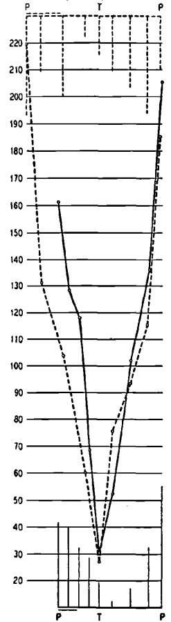
Freight car orders --- First group (5 cycles) — Last group (4 cycles)*
