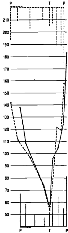
Shares traded --- First group (5 cycles) — Last group (5 cycles)
