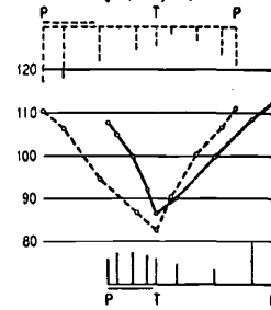
Railroad stock prices --- First group (5 cycles) — Last group (5 cycles)
