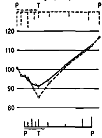
Deflated clearings --- First group (5 cycles) — Last group (5 cycles)
