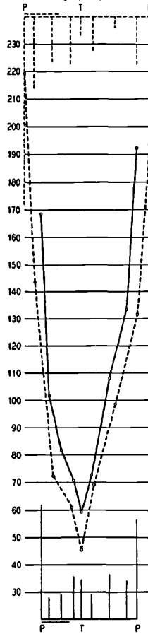
Call money rates --- First group (5 cycles) — Last group (5 cycles)
