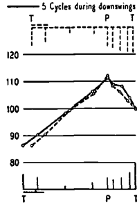
Deflated clearings --- 7 Cycles during upswings --- 5 Cycles during downswings
