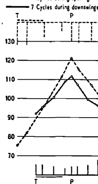
Railroad stock prices --- 7 Cycles during upswings --- 7 Cycles during downswings
