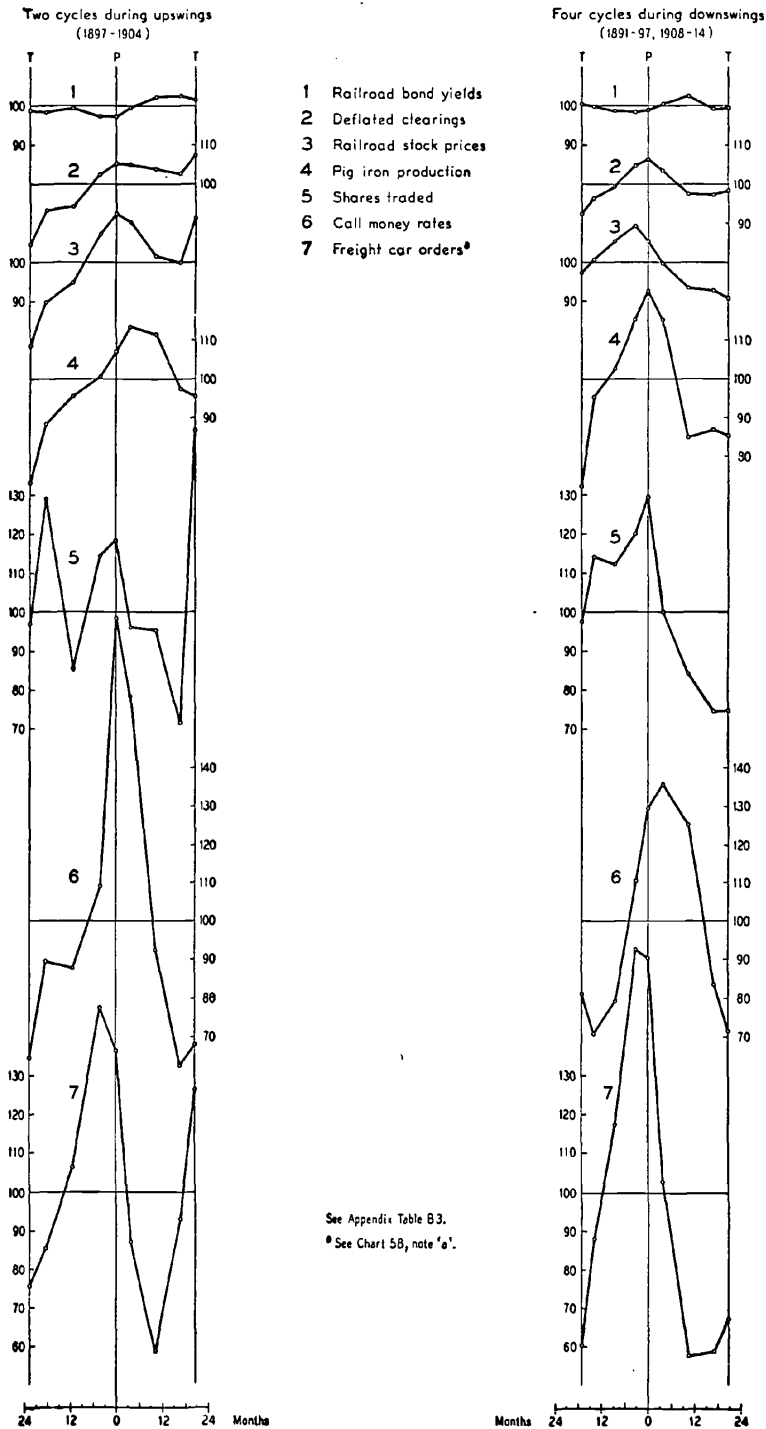
CHART 62 Average Reference-cycle Patterns during the Upswings and Downswings of Wardwell's Major Cycles, 1891-1914 Seven American Series
