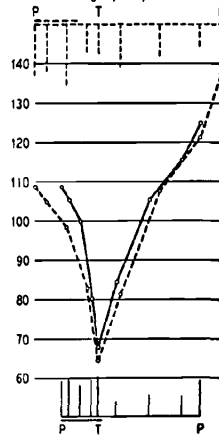
Pig iron production --- First group (5 cycles) — Last group (5 cycles)
