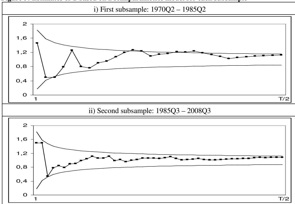
Figure 5: Estimates of d based on a semiparametric model for each subsample
