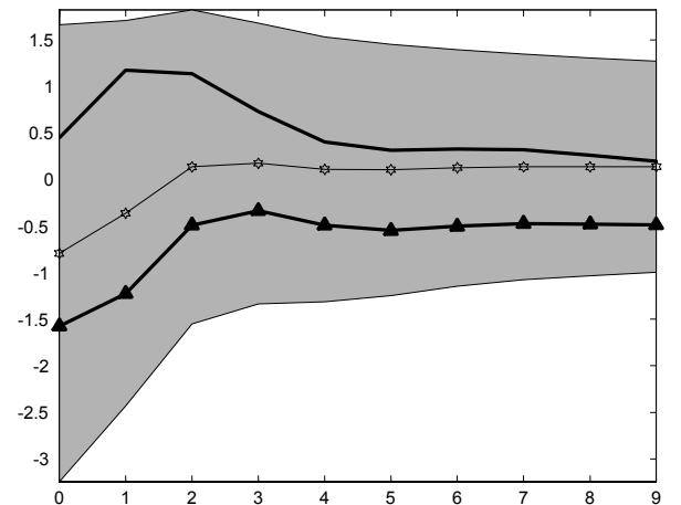
Panel B: DGP - Difference VAR
