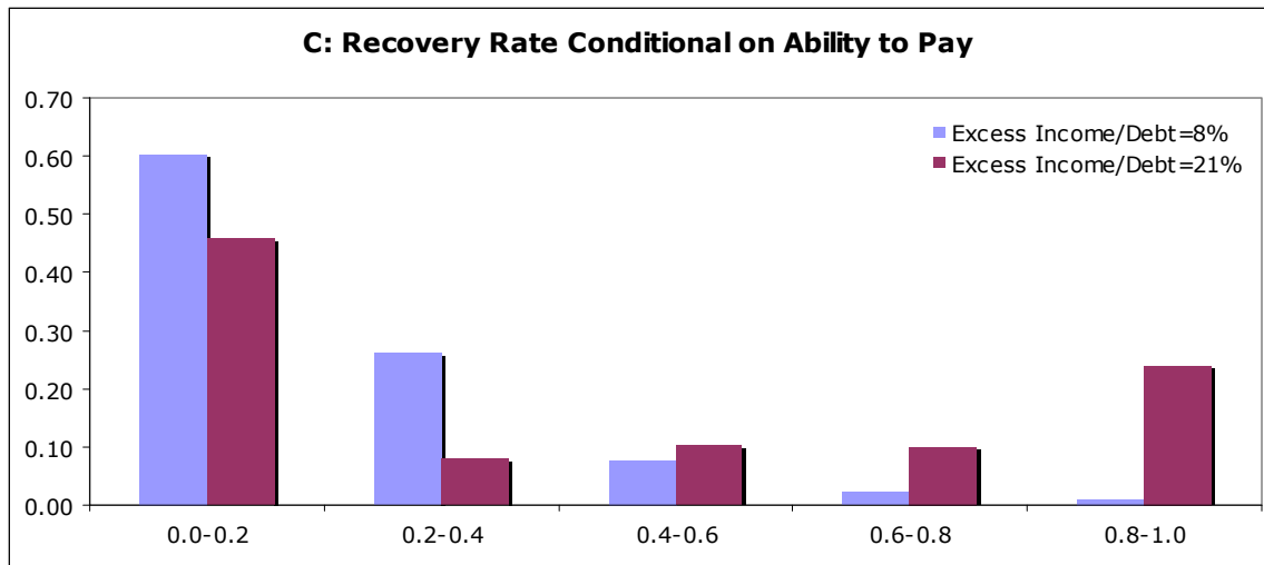
Figure 6: Model-Generated Conditional Distributions of Recovery Rates
