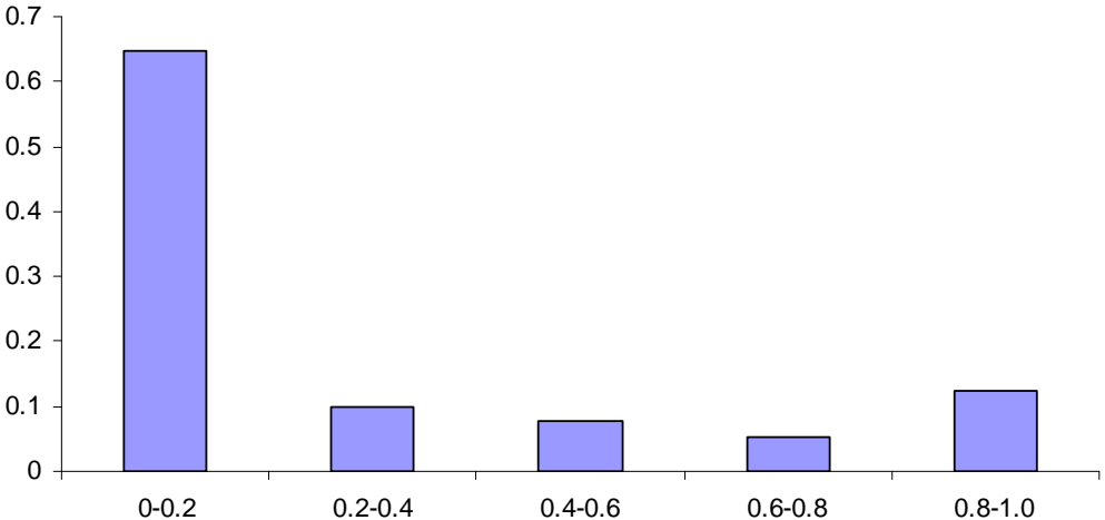
Figure 2: Distributions of Recovery Rates
