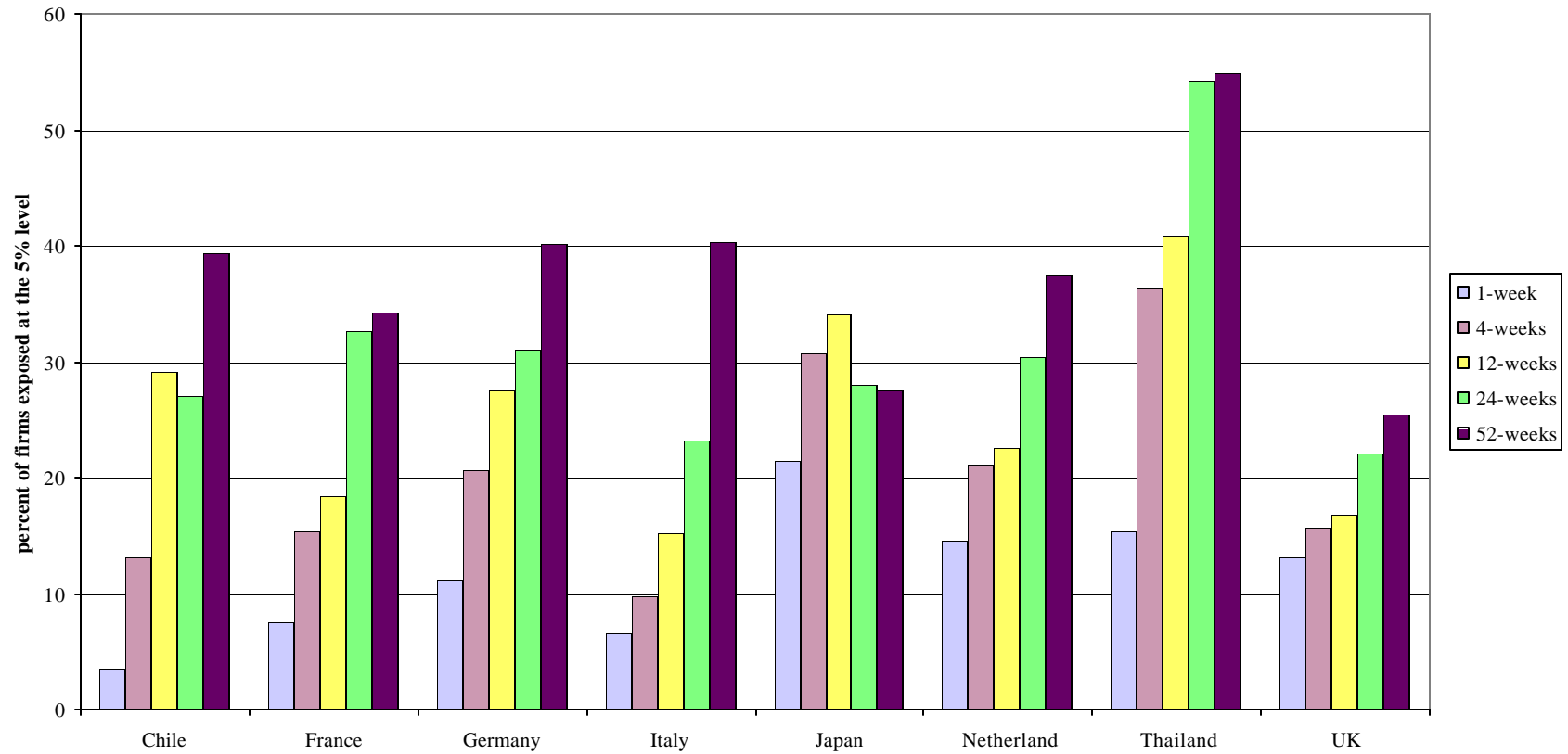
Figure 4 -- Sensitivity of Exposure to Return Horizon
