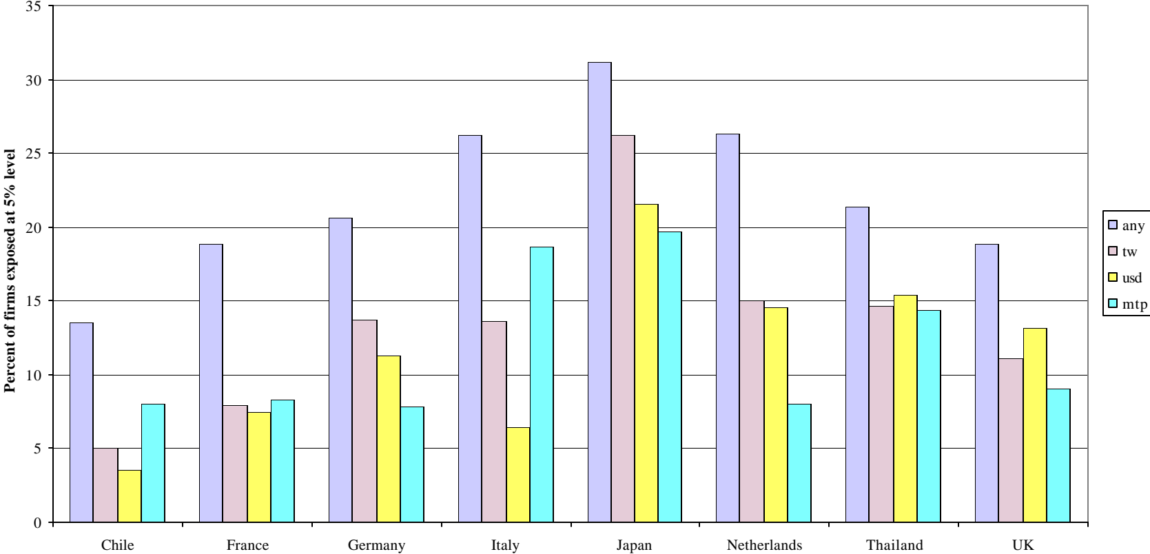
Figure 1 -- The Sensitivity of Exposure to Different Exchange Rates
