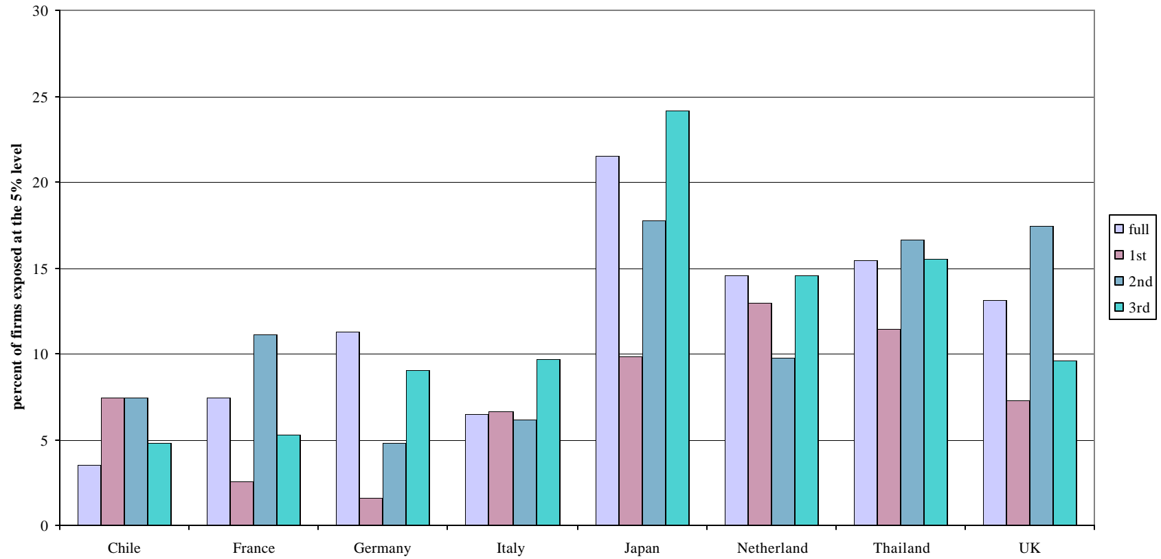
Figure 5 -- Robustness of Exposure Across Subsamples
