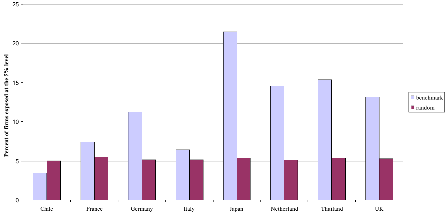
Figure 3 -- Exposure or Spurious Correlation?
