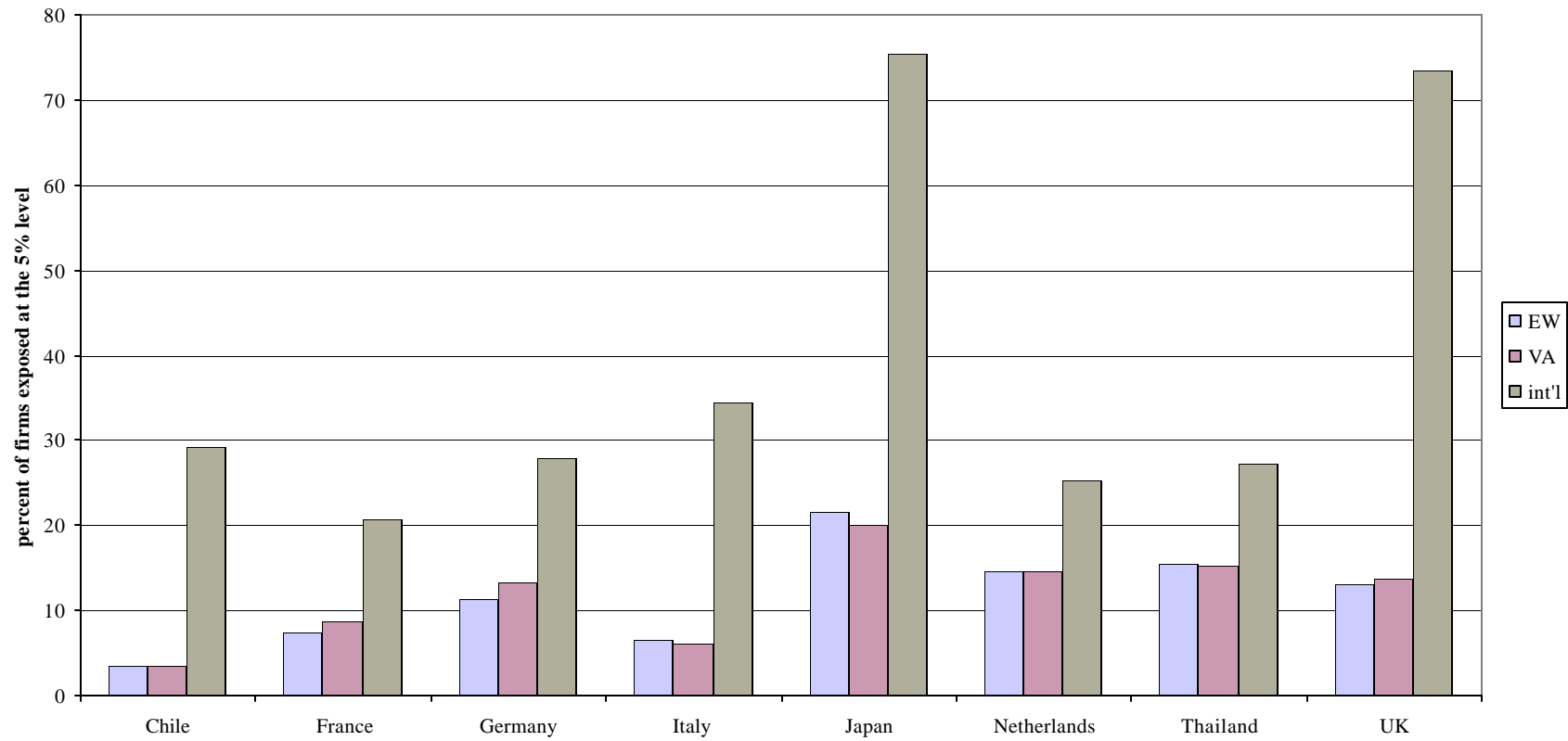
Figure 2 -- Sensitivity of Exposure to Choice of Market Index
