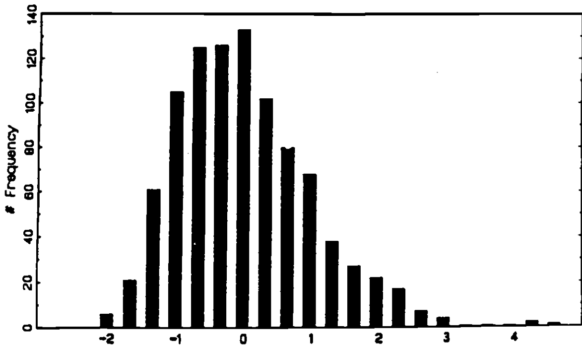
Figure 9b: Histogram of Structures V/K (standardized)
