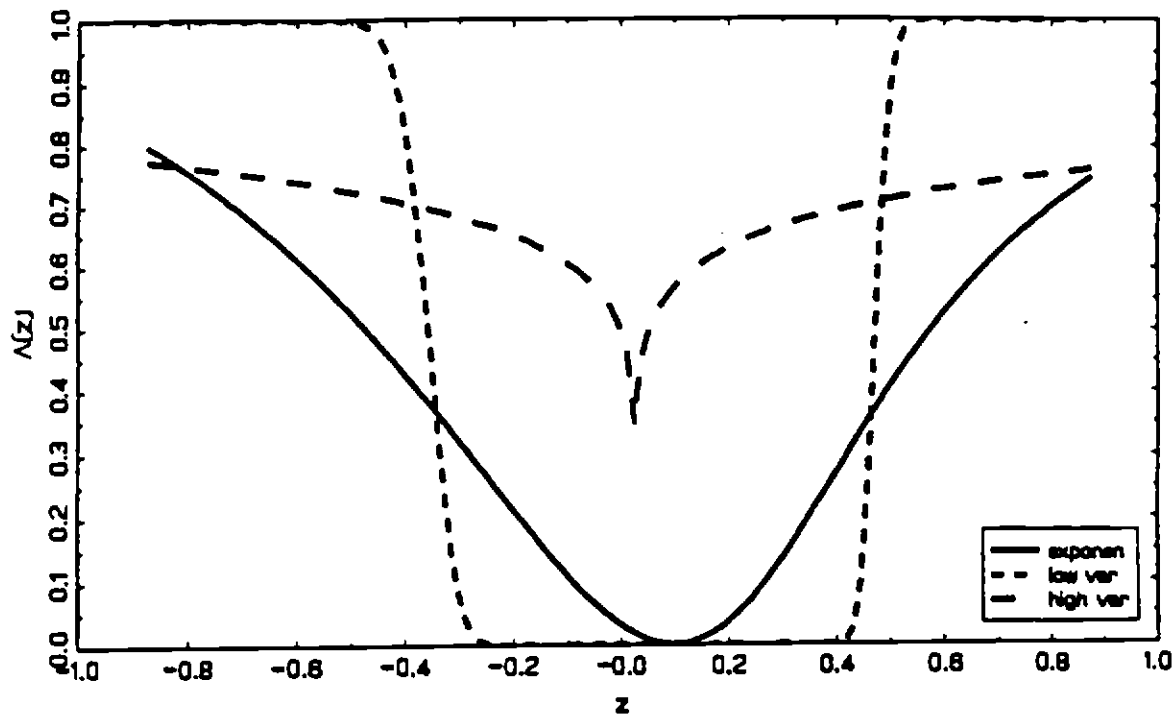
Figure 4b: Adjustment costs
