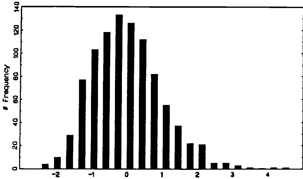
Figure 9a: Histogram of Equipment V/K (standardized)
