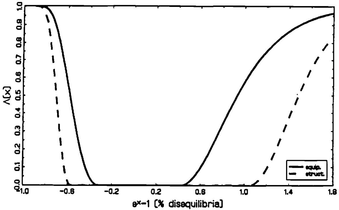
Figure 6b: Distributions of adjustment costs
