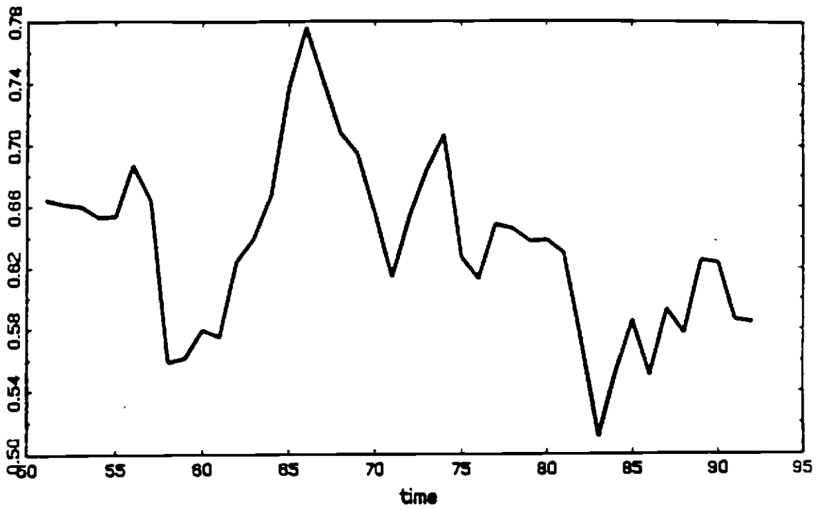
Figure 7b: Structures-index of responsiveness
