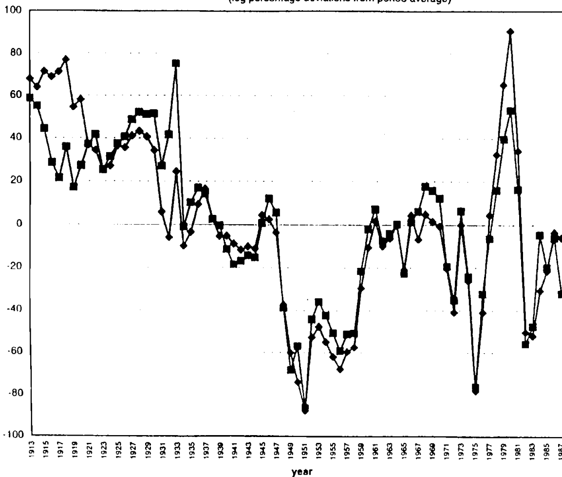
Figure 1 Real Value of the Argentine Austral 1913-1988 (log percentage deviations from period average)
