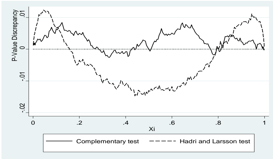
Figure 3. P-value Discrepancy for the two tests.
