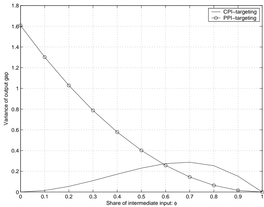
Figure 3:—The variance of output gap under extreme inflation-targeting policies.
