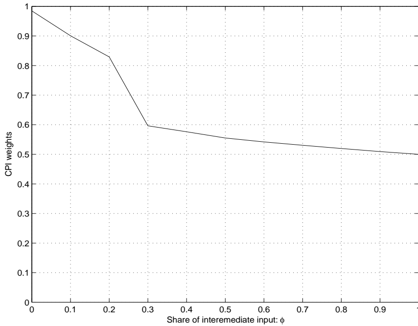
Figure 2:—The weight on CPI inflation in the optimal inflation index.
