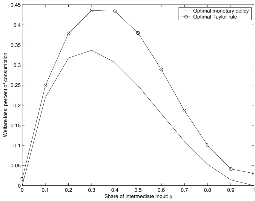
Figure 1:—Sensitivity of welfare losses to the share of intermediate input.
