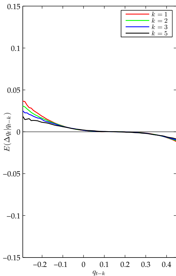
(a) k = 1, 2, 3, 5 .
