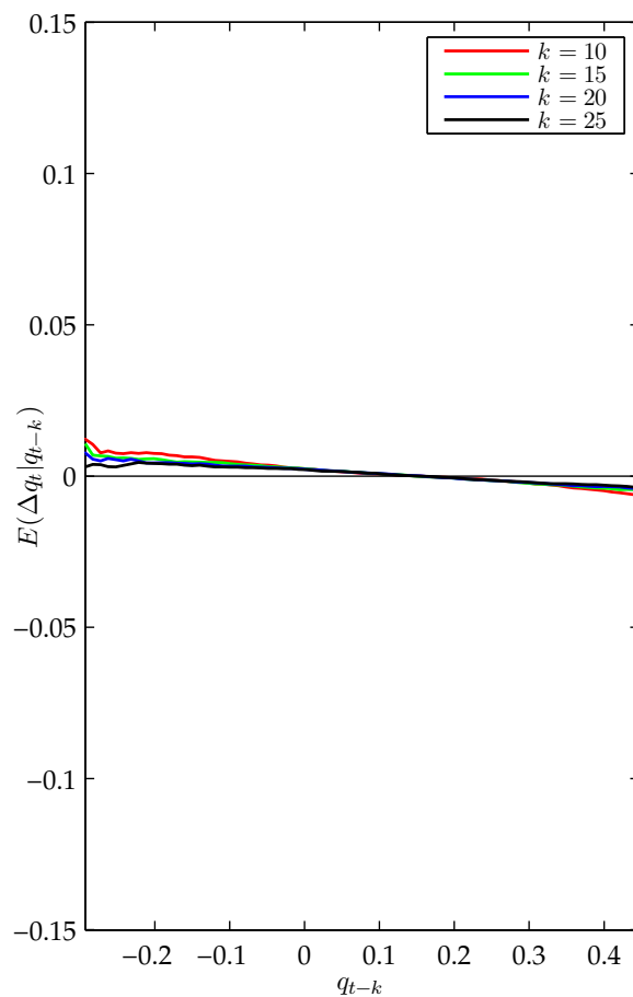
(b) k = 10, 15, 20, 25 .
