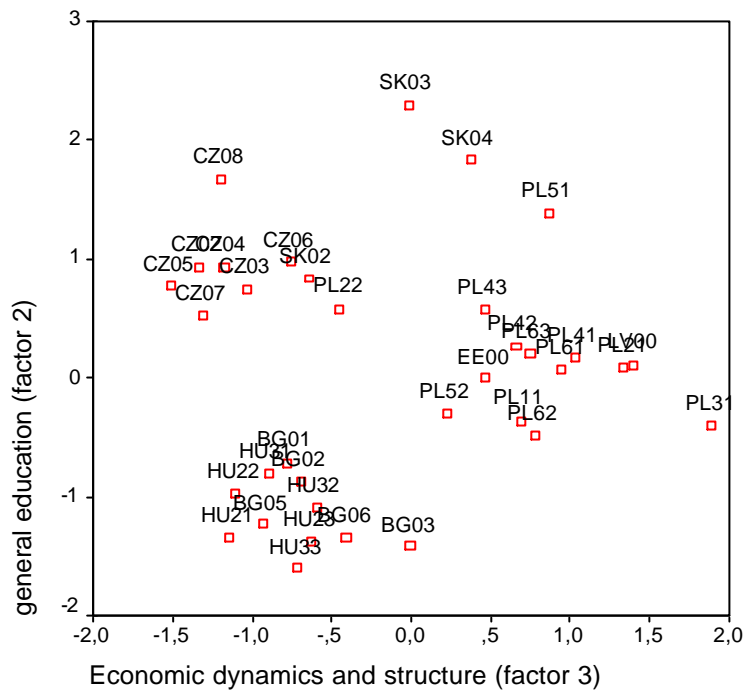
Figure 3: The 38 remaining regions plotted on factors 2 and 3
