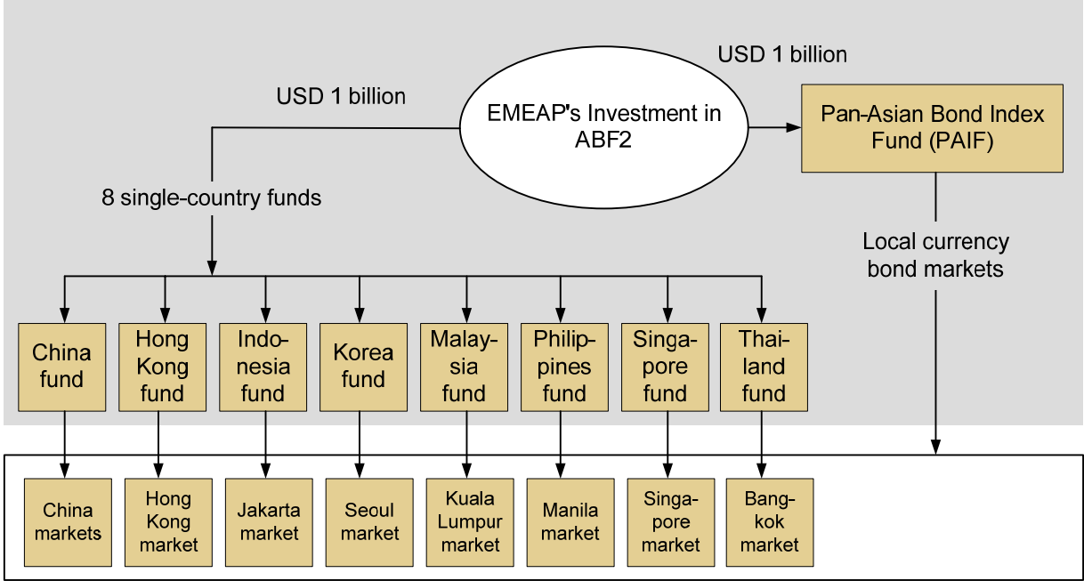
Figure 2: ABF2 Structure
