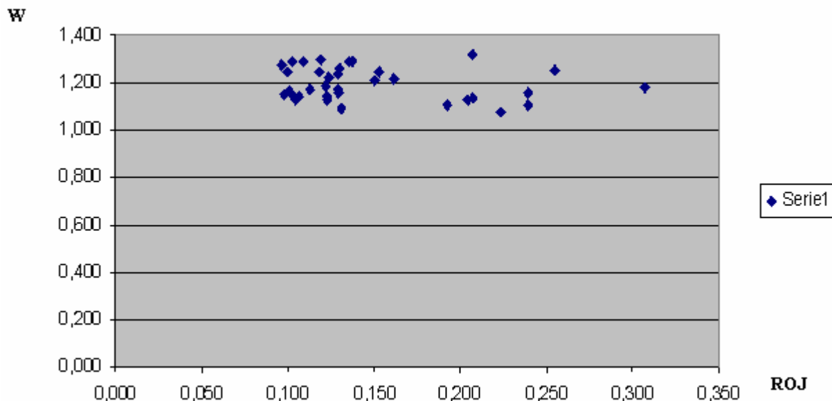
Fig. 6 Reference points in \langle W - ROJ \rangle space
