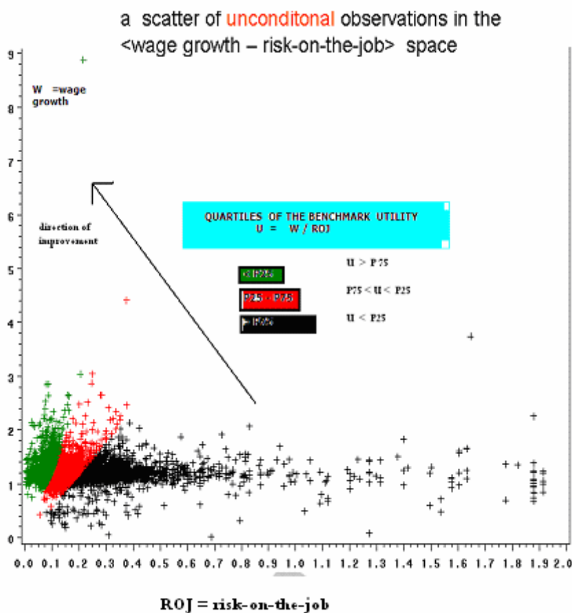
Fig. 1 Scatter of unconditional observations in the <W- ROJ > space
