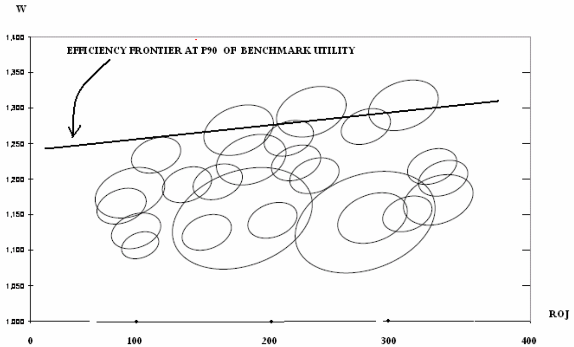
Fig. 7 Reference points y^* - centered ellipses in \langle W-ROJ \rangle space
