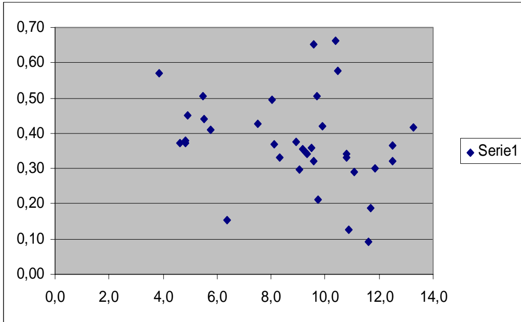
Fig. 8 : D(k) in the ordinate, U[y^*(k)] in the abscissa.
