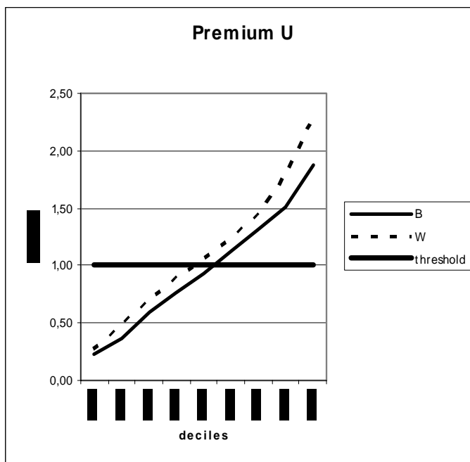
Fig. 8 A quasi counterfactual analysis: Premium Utility = W / ROJ
