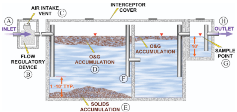
Figure 7. Grease Interceptor
