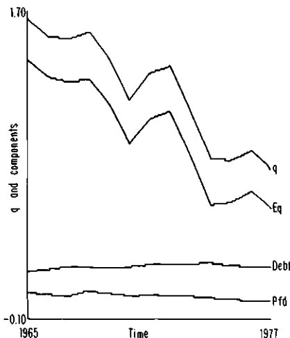
Fig. 2.4 q and components, 1965-77.
