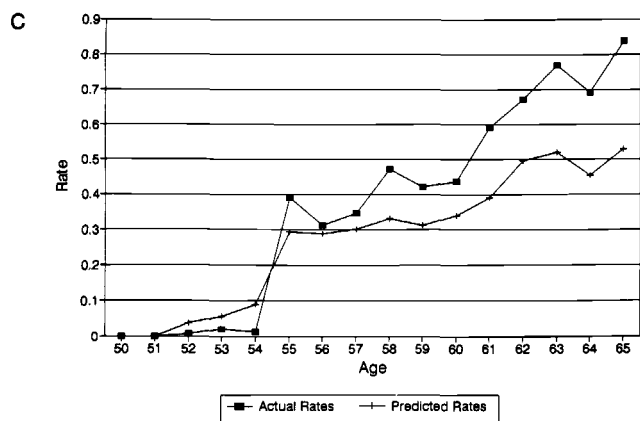
Fig. 6.13 Predicted vs. actual (A) annual departure rates, (B) cumulative departure rates, and (C) window departure rates: men and women, SDP, Medicare
