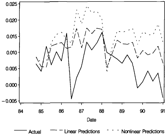
Fig. 8.1 Postsample forecasting performance of the model
