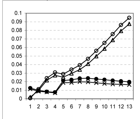
FIG. 3. DIRECT AND INDIRECT FORECASTS OF THE M2 VELOCITY(V2): AR MODELS Cumulative Root Mean Squared Error
