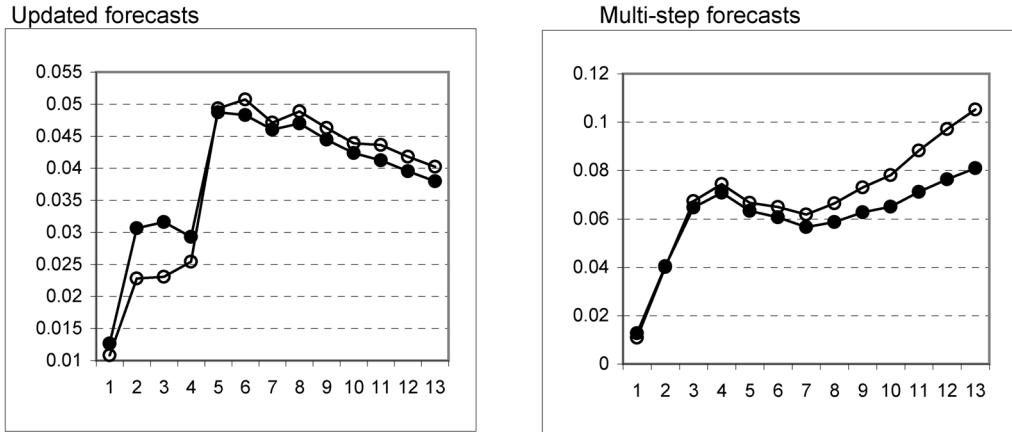
FIG. 4. DIRECT AND INDIRECT FORECASTS: HARVEY'S MODEL
