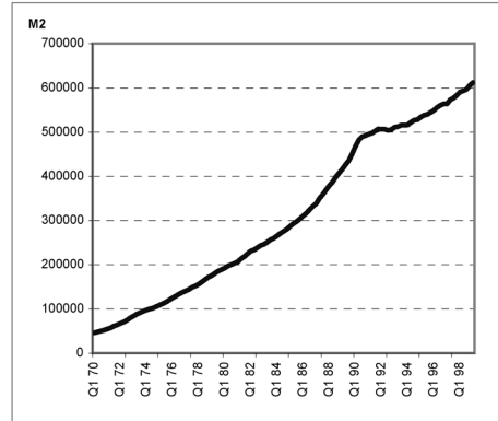
FIG. 1. TIME SERIES PLOTS OF THE VARIABLES
