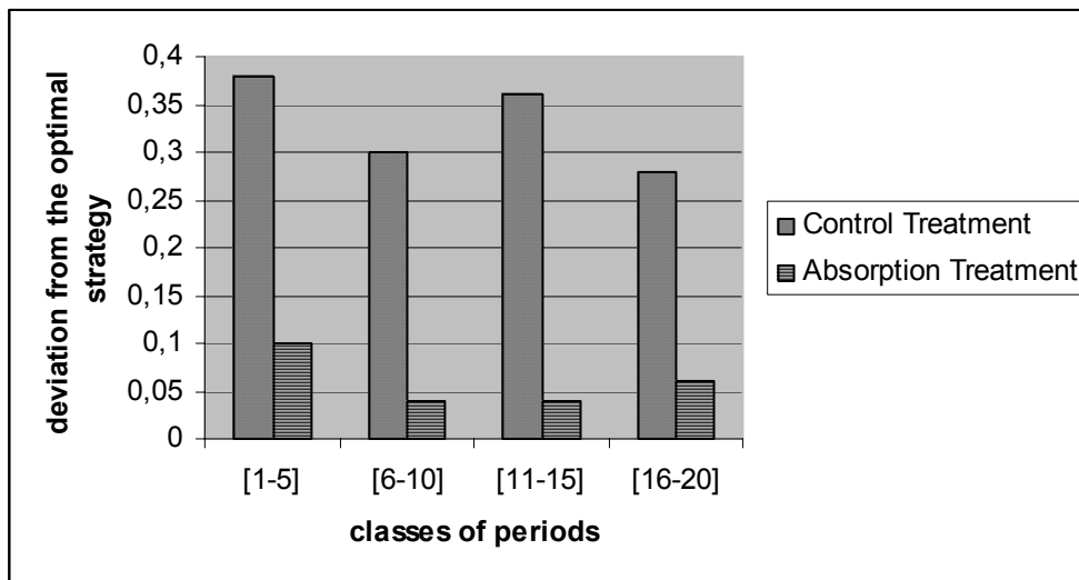
Figure 5: Average percentages of deviant strategies per classes of periods
