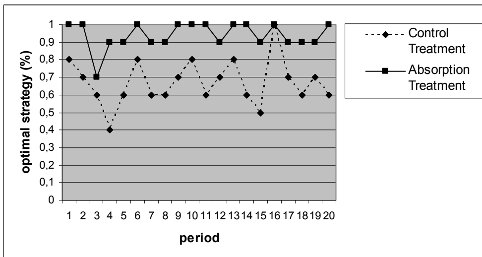
Figure 4: Percentages of optimal strategy per treatment
