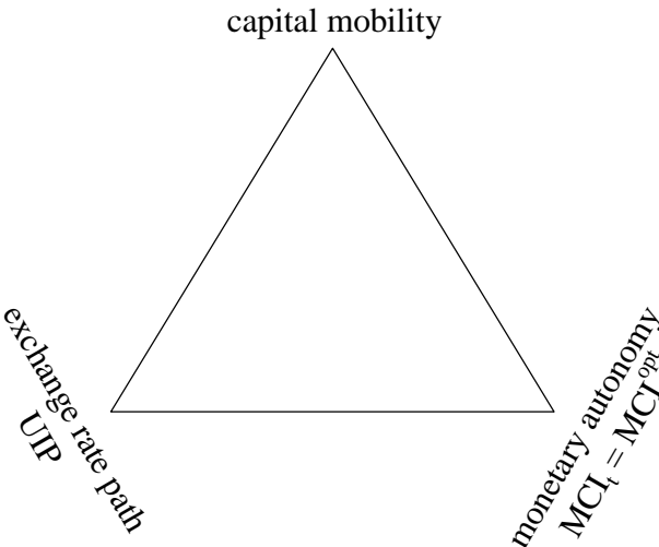
Figure 8: Consistency triangle
