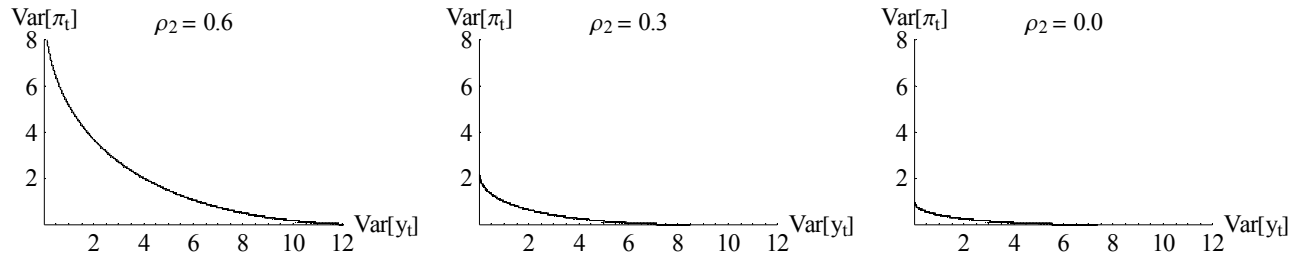
Figure 2: Efficient frontiers
