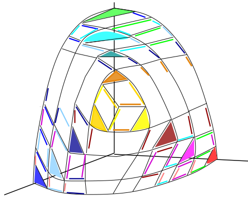
Figure 2.5: The general cephoid in \mathbb{R}^3
