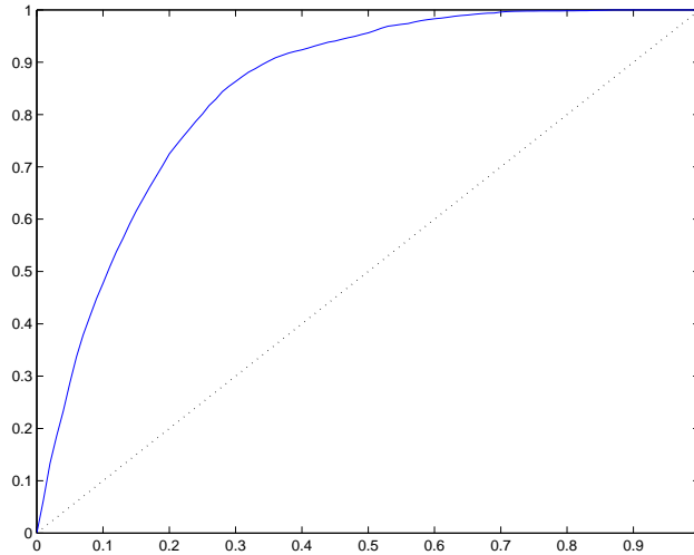
Figure 9: Average out-of-sample power curve for 5-year default prediction, January 1993 to December, 1999.
