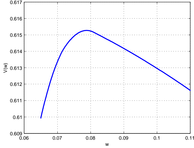
Figure 1: Theorem 3 part 2. Value function with \beta = \delta = 0.9 .
