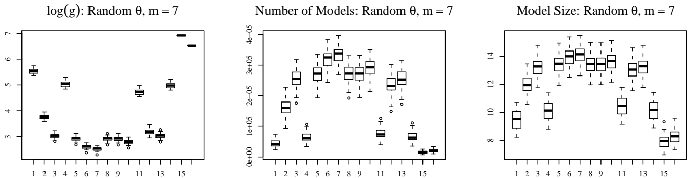
Fig. 10. Tobias-Li data: log posterior medians of g , number of models visited and posterior mean model size.
