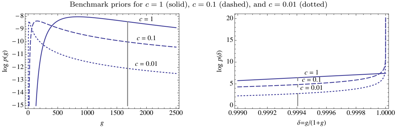
Fig. 1. Beta Benchmark Priors for g and \delta ( n = 72 , k = 41 )
