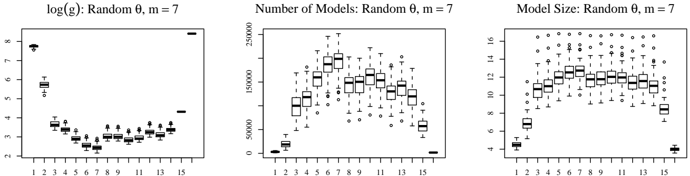
Fig. 9. SDM data: log posterior medians of g , number of models visited and posterior mean model size.
