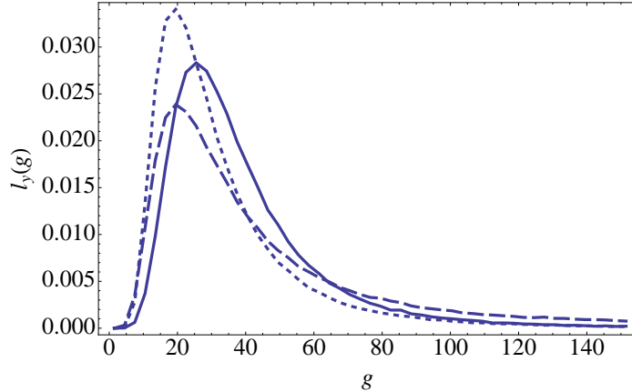
Fig. 8. Marginal likelihood l_y(g) : FLS (solid), SDM (dashed) and Tobias-Li (dotted) data (random \theta , m = 7 )
