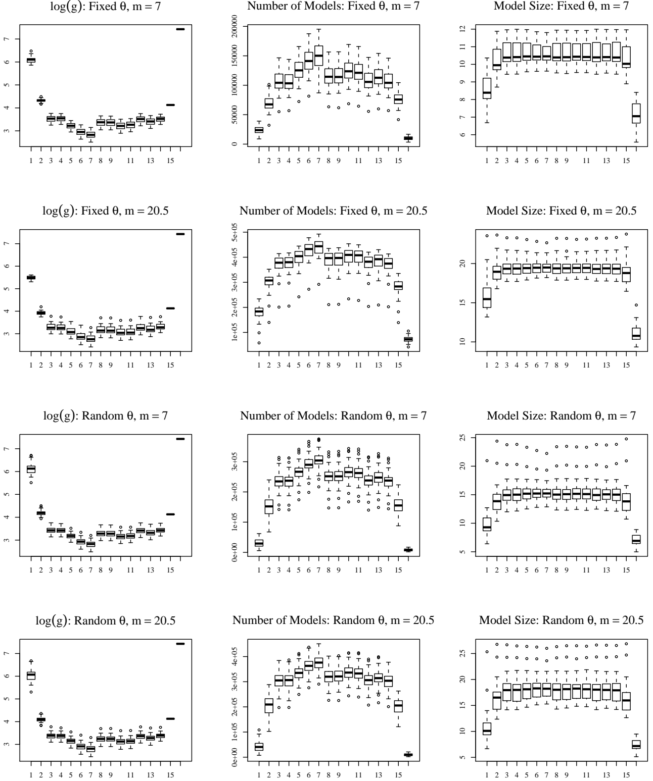
Fig. 6. FLS data: log posterior medians of g , number of models visited and posterior mean model size The different priors on g are ordered as in Tables 2 and 3. The top two rows correspond to fixed \theta (with different m ), while the bottom two rows are for random \theta priors on model space
