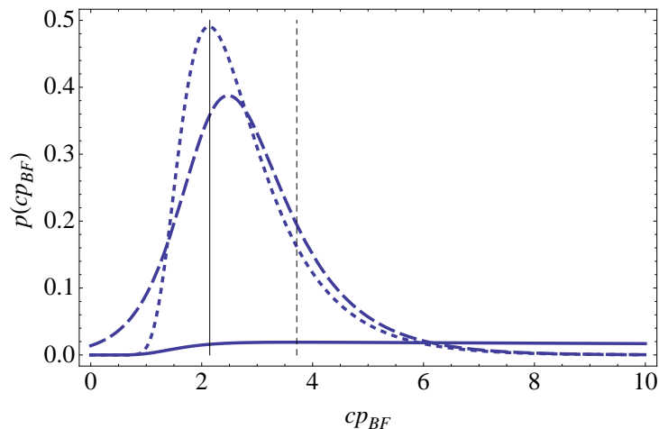
Fig. 4. Prior of complexity penalty cp_{BF} ( n = 72, k = 41 )
