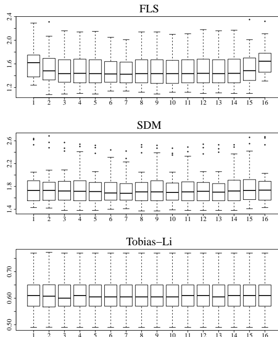
Fig. 7. Log Predictive Score: FLS, SDM and Tobias-Li data (random \theta , m = 7 )
