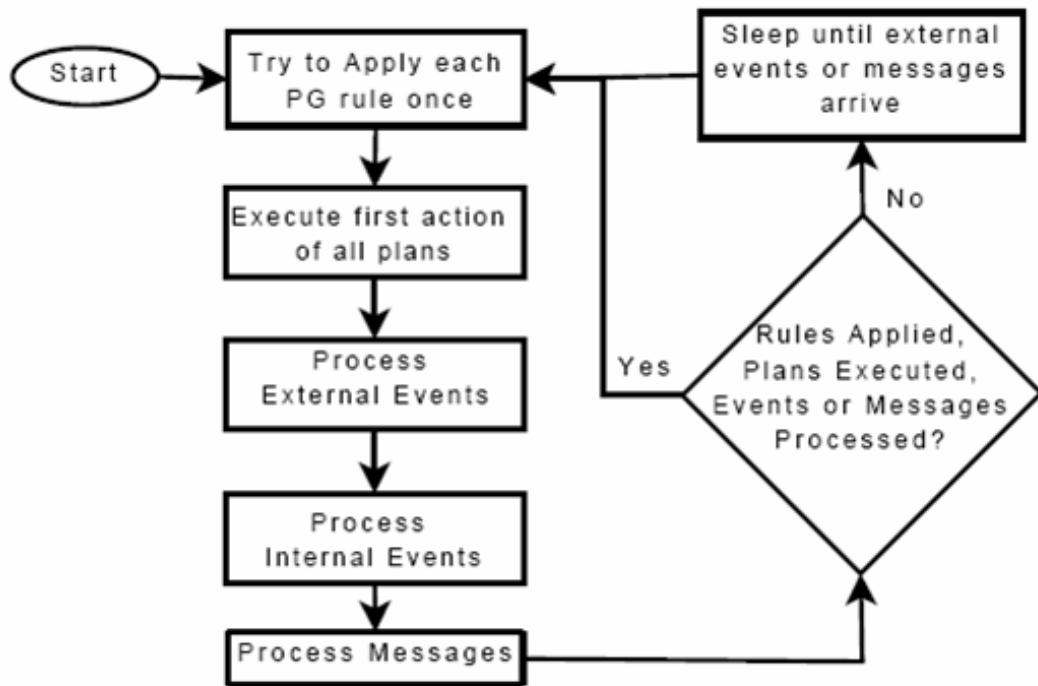
Figure 2. The deliberation cycle of a 2APL agent
