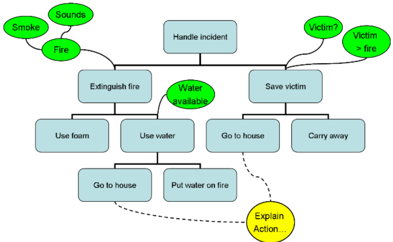
Figure 1. BDI-model of a firefighter agent
