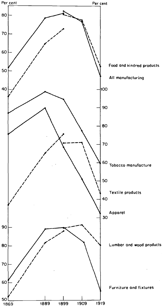
Share of Steam in Primary-Power Capacity in All Manufacturing and in Each Industry Group, 1869-1919
