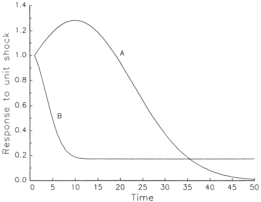
Figure 1 IMPULSE-RESPONSE FUNCTIONS
