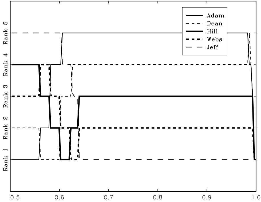
Figure 2. Ranking of the methods according to \bar{\alpha} for year 1870 ( k = 2 )
