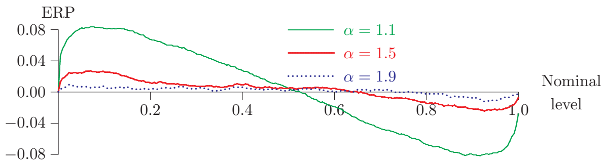
Figure 13: P value discrepancy plots, \hat{\alpha}_{\text{Hill}} , \hat{\beta}_{\text{AM}} , stable law
