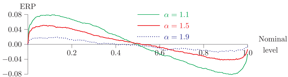
Figure 12: P value discrepancy plots, \hat{\alpha}_{Hill} , \hat{\beta}_{Hill} , Student's t law
