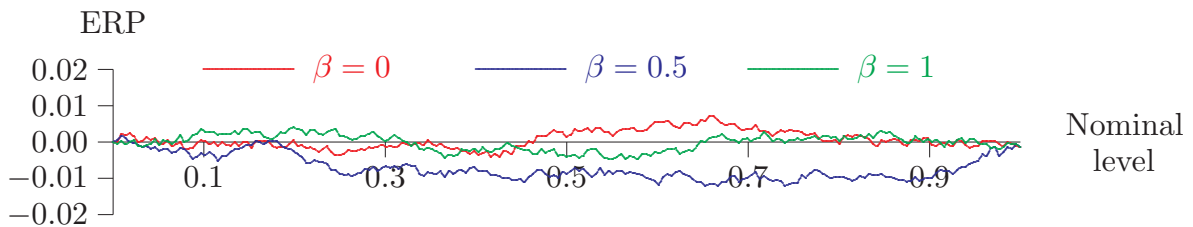
Figure 6: P value discrepancy plots, \alpha = 1.5 , n = 100
