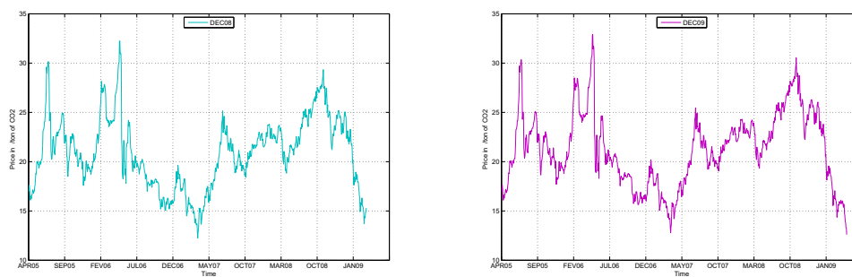
Figure 1 Carbon futures prices of maturities December 2008 (left) and 2009 (right) from April 22, 2005 to January 16, 2009
