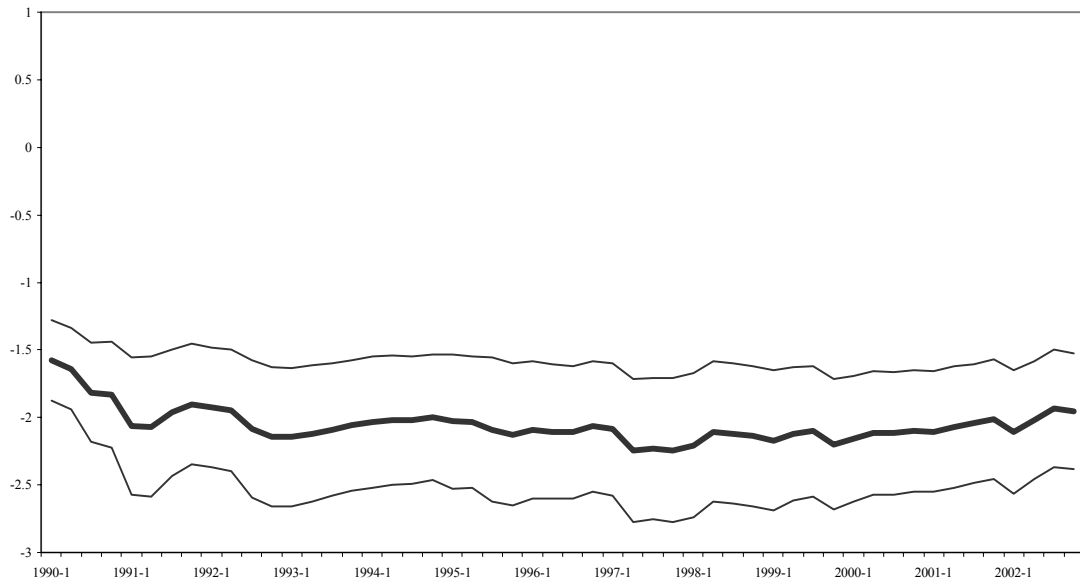
Figure 5: Recursively estimated market share coefficient in the R&D-intensity vector and +/- 2SE bands – Cross-equation restriction imposed
