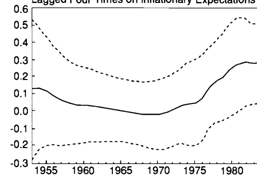
Recursive Regression Estimates of Effect of Inflation Lagged Four Times on Inflationary Expectations
