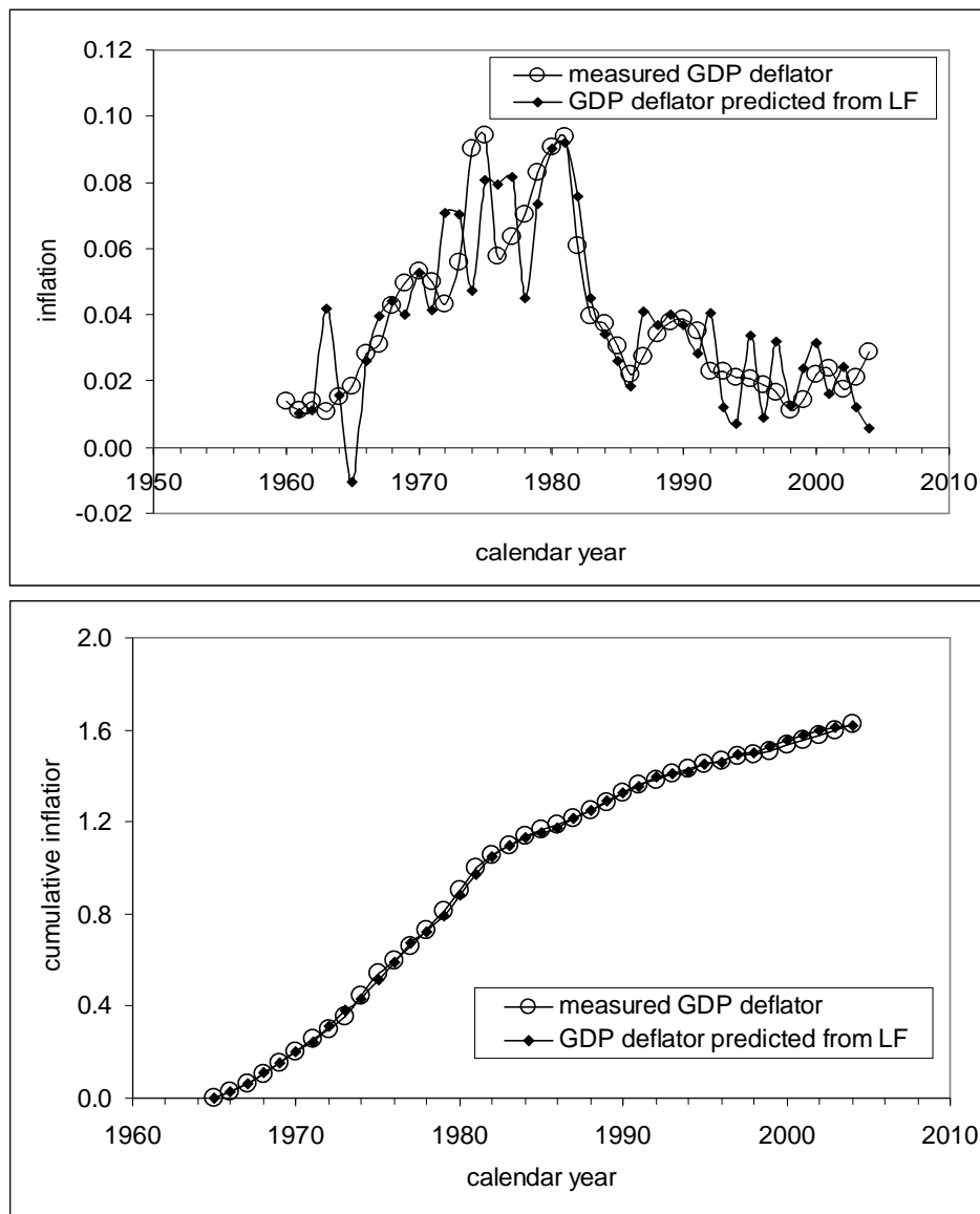
Figure 8. Observed and predicted inflation (GDP deflator). The predicted values are obtained using Eq. (13) with a_1=4.0 , a_2=-0.3 , and T_1=2 years. The upper panel compares annual readings and the lower one – cumulative values.
