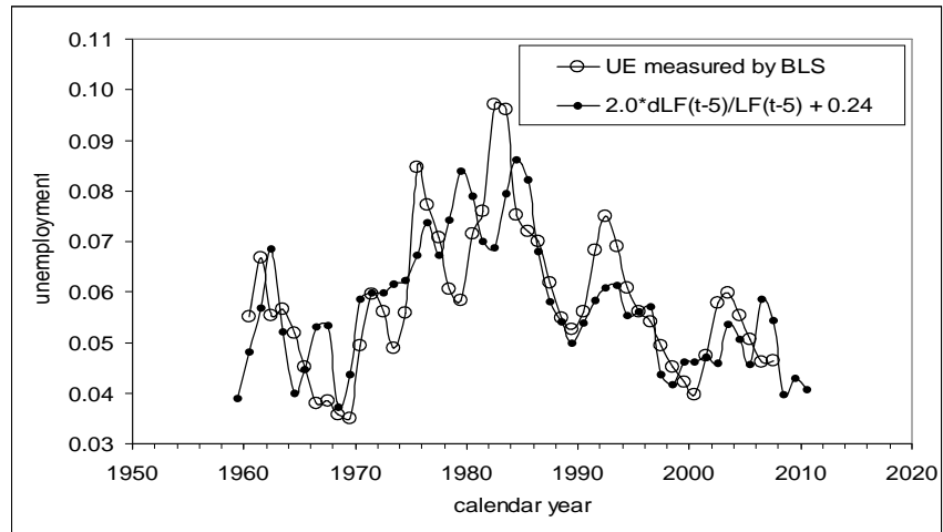
Figure 10. Observed and predicted unemployment rate. The latter is obtained from the estimates of the labor force in the US between 1960 and 2006. The 5-year lag of the unemployment behind the labor force allows a prediction of unemployment up to 2011. Notice a local peak in the predicted curve near 2008.
