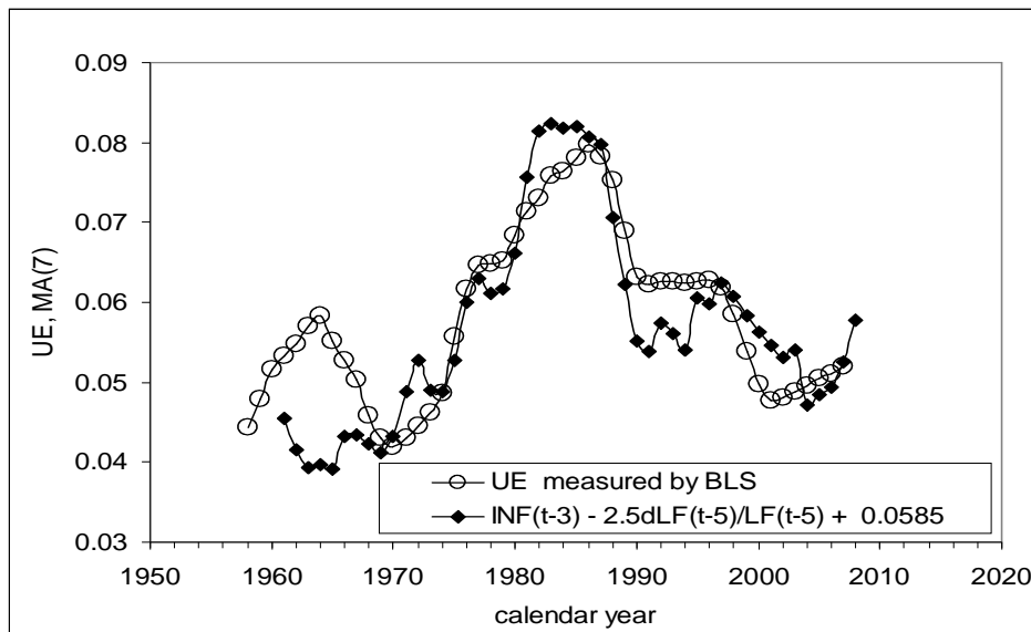
Figure 13. Same as in Figure 12, but smoothed by MA(7). There are some weak deviations (approximately 0.5 %) between the smoothed curves in the 1990s and the beginning of the 2000s.
