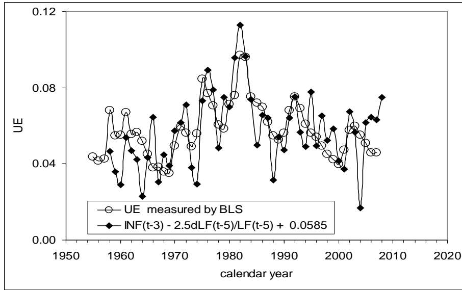
Figure 12. Unemployment measured by the BLS and that predicted as a lagged linear function of labor force change rate ( dLF/LF ) and inflation ( INF ) represented by GDP deflator: UE(t) = \pi(t-3) - 2.5dLF(t-5)/LF(t-5) + 0.0585.
