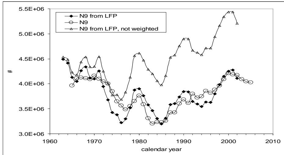
Figure 3. The number of 9-year-olds: the observed one and that obtained from the LFP with and without exponential weighting in (5). Constants t_0=1963 ; B_2=-1.5E+8 , C_2=4.94E+6 , \alpha_2=-1.85 . The case with \alpha_2=0 in also shown: N_9 is highly overestimated.
