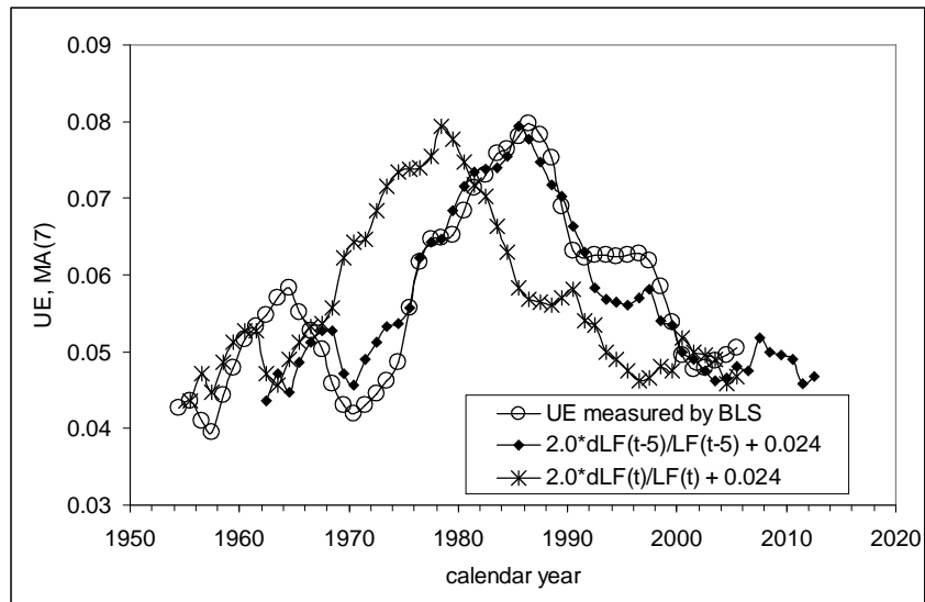
Figure 10. Observed and predicted unemployment rate. The latter is obtained from the estimates of the labor force in the US between 1960 and 2006. The 5-year lag of the unemployment behind the labor force allows a prediction of unemployment up to 2011. Notice a local peak in the predicted curve near 2008.
