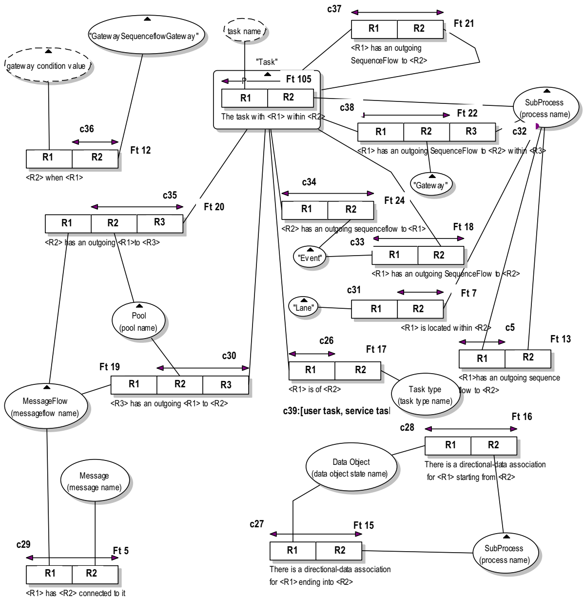
Fig 17c. Information Structure diagram for BPMN palette 1 modeling constructs including constraints (III).
