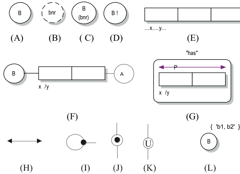
Fig. 1. Main notation symbols in the ORM fact-Oriented dialect
