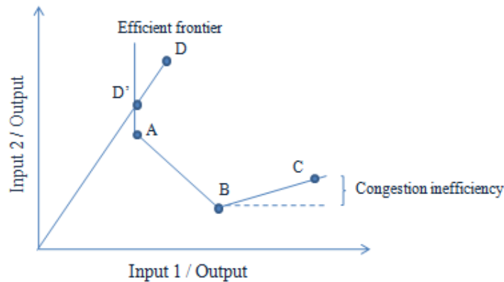
Figure 1 DEA Efficient frontier and congestion inefficiency
