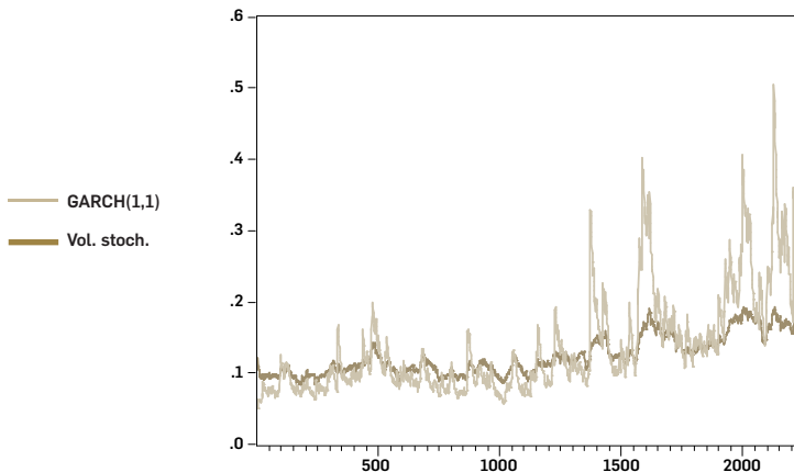
Figure 7. Annualized stochastic volatility and GARCH(1,1) volatility, S&P/TSX return, 1992-2000.
