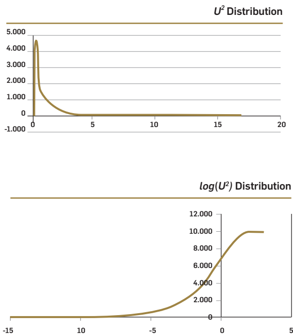
■ Figure 1. Distributions of U^2 and of \log(U^2) , U \sim N(0,1)
