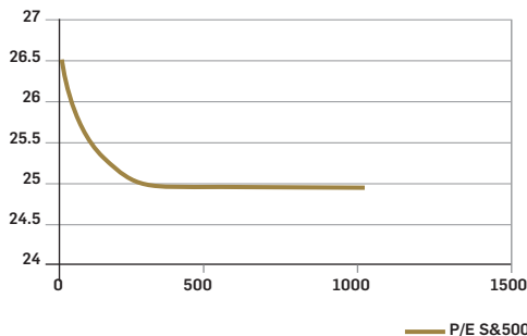
■ Figure 9. (P/E) simulation from its value in May 2005 to its steady-state value
