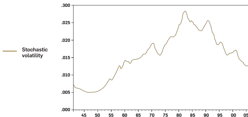
■ Figure 4. Stochastic volatility of the Canadian T-bill yield.
