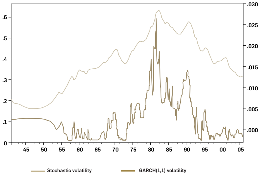
Figure 5. Annualized, stochastic volatility and GARCH(1,1) volatility, Canadian T-Bill yield, 1941-2005.
