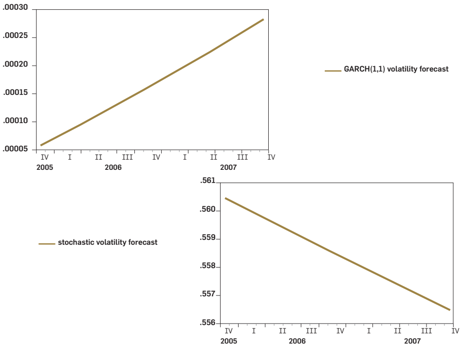
■ Figure 8. Volatility forecast, stochastic model and the GARCH(1,1) model, Canadian Treasury bill yield.
