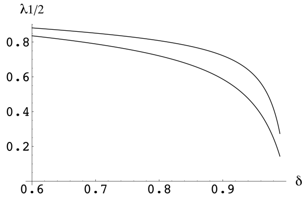
Figure 1: \lambda_{1/2} as a function of \delta for c = .65 and .85 .
