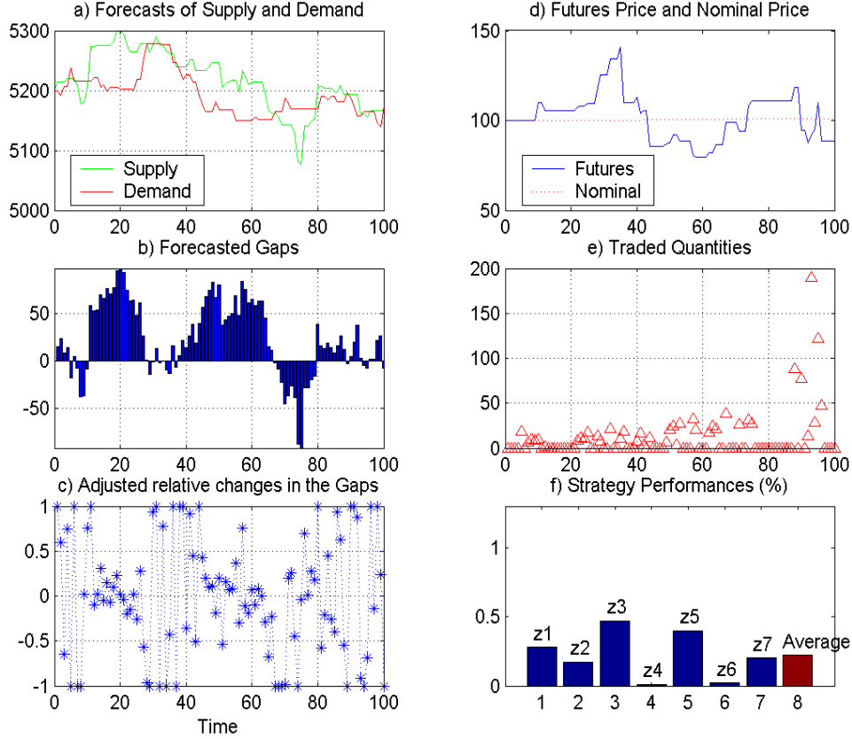
Figure 4: Pricing obtained by the automatic trading strategy
