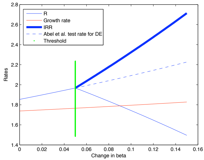
Figure 4: Steady states and technological transition
