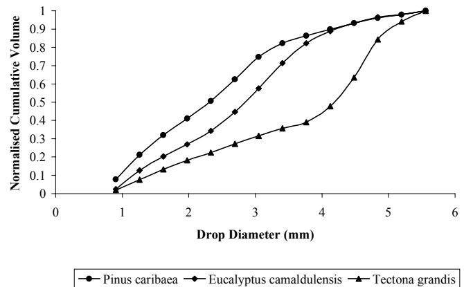
Fig. 5 Characteristic net-rainfall drop-size spectra for Pinus caribaea , Eucalyptus camaldulensis and Tectona grandis (from Hall and Calder, 1993)
