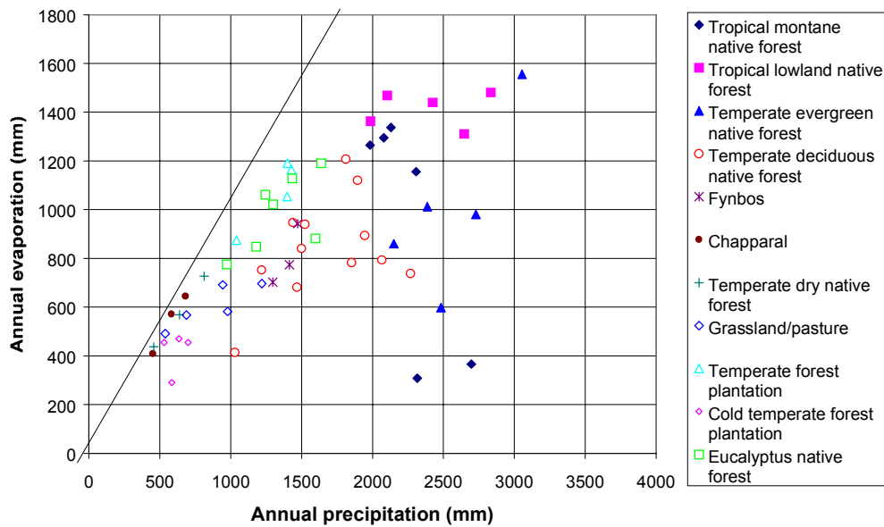
Fig. 3 Annual evaporation plotted against annual precipitation for different vegetation types from different regions of the world
