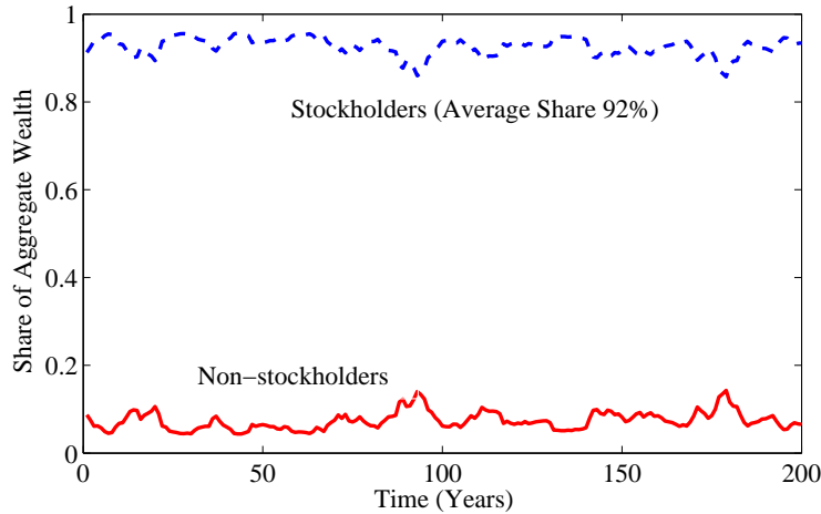
Figure 6: Evolution of wealth distribution over time
