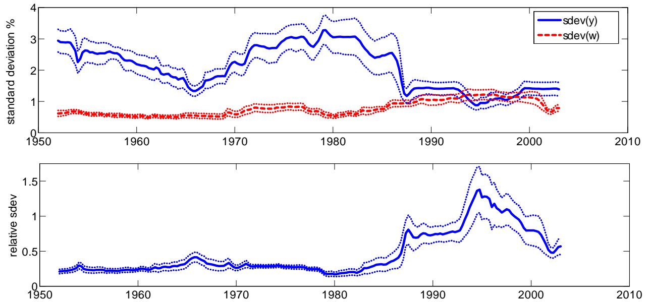
Figure 1: Rolling windows of standard deviations (upper panel) and relative standard deviations (lower panel). Dotted lines represent \pm one standard deviation bands.
