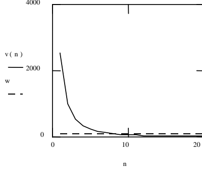
Fig 2.1-Values of v^*(n) and \bar{w}=\bar{v} for a=350 and n=1, \dots, 20 . In this example v^*(n) is equal to \bar{v}=10 for \underline{n}=8 .
