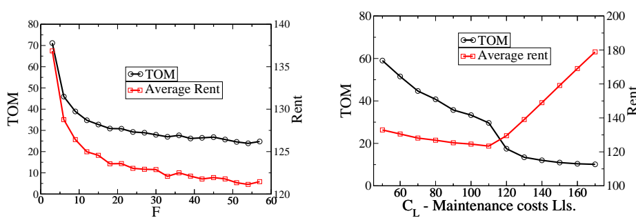
Figure 19: Left : The variations in average rent and the average TOM as a function the length of landlords' memory. Right : The variations in average rent and the average TOM as a function of landlords' maintenance costs.
