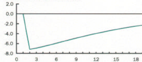
I. Transactions balances ( \bar{Q} ) percent deviation from steady state
