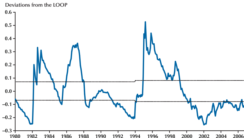
Figure 1 Footwear Real Exchange Rate and Threshold Bands
