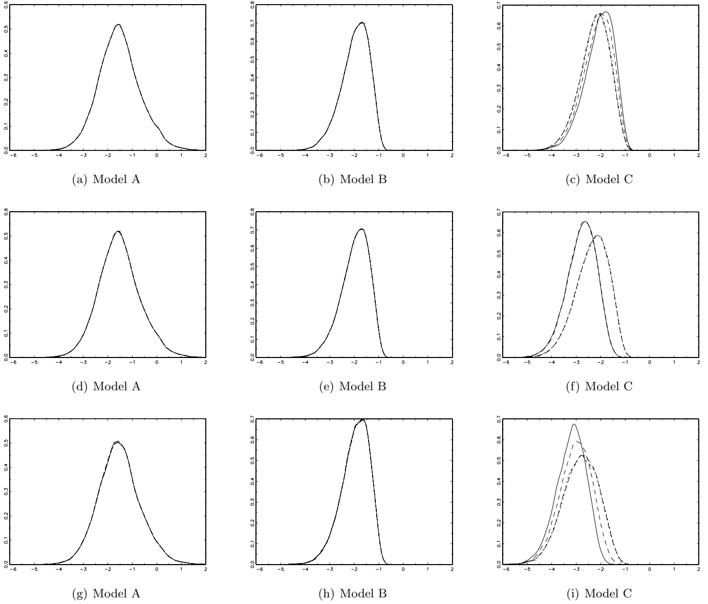
Figure 3: Asymptotic Densities of WE_{t-stat} Statistic.
