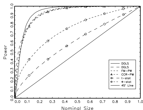
(f) \alpha_1 = 1, \delta = 0.5
