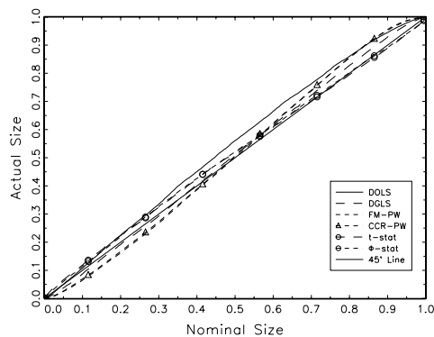
(b) \alpha_1 = 1, \delta = 0.5
