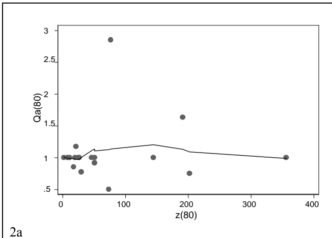
Figure 2: The Global effect of energy consumption on countries' economic efficiencies
